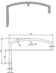
45 x 90 Pervaz Oval 45 x 90 Case Oval
